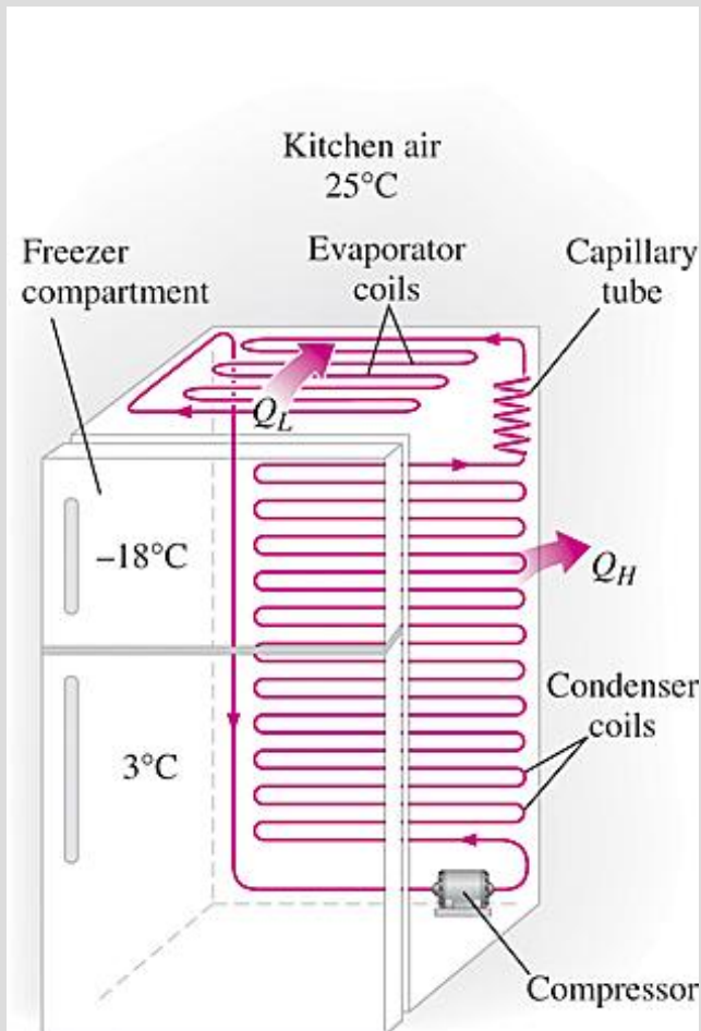
An ordinary household refrigerator.
